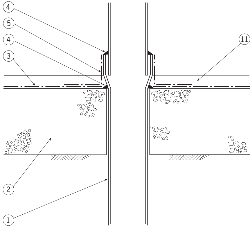
Soil vent pipe entry
